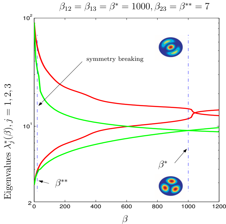
Fig. 6. Bifurcation of \theta - and radial-symmetry ( m = 3 ).
