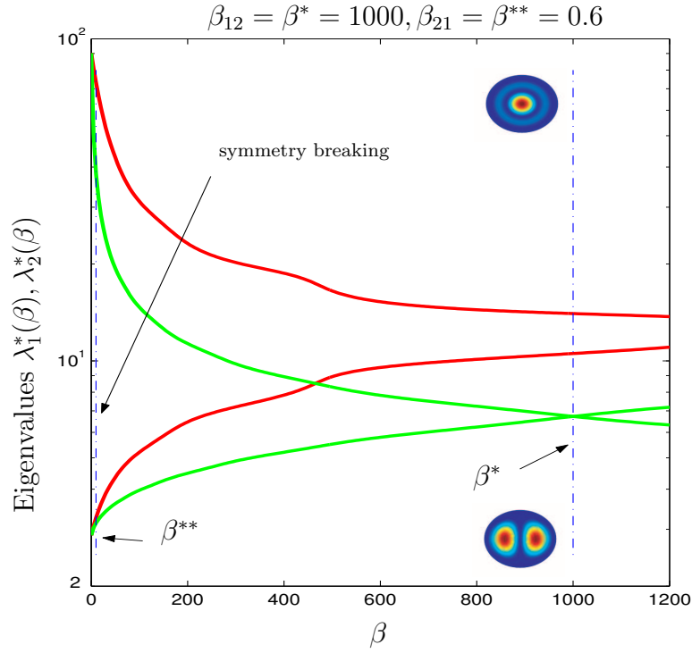
Fig. 5. Bifurcation of \theta - and radial-symmetry ( m = 2 ).
