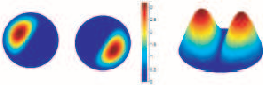
(a) green: \beta^* = 1000 , \lambda_1^* = \lambda_2^* = 7.07 , E(\mathbf{u}^*) = 7.02
