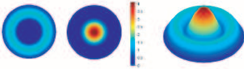
(b) red: \beta^* = 1000 , \lambda_1^* = 10.34 , \lambda_2^* = 14.54 , E(\mathbf{u}^*) = 12.43
