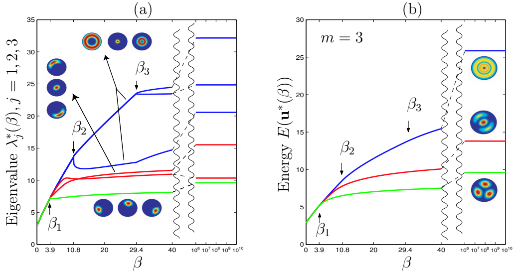
Fig. 2. (a): Eigenvalue curves, (b): energy curves, vs \beta .
