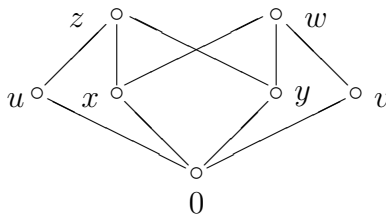
Figure 3. A pooling space which is not a meet semi-lattice.
