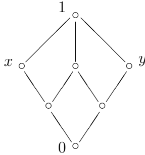
Figure 2. An upper semi-modular lattice that is not lower semi-modular.
