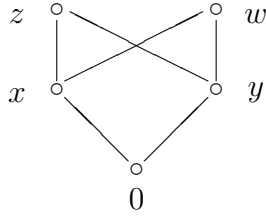
Figure 1. A poset.
