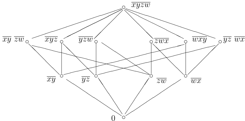
Figure 4. The poset P(C_4) of contractions of C_4 . P(C_4) is upper semi-modular, but not lower semi-modular.
